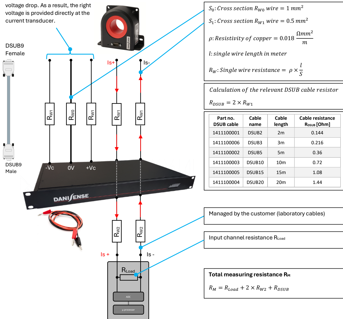
Figure 5: Calculation scheme for the cable resistances and the total measuring resistance R_M
