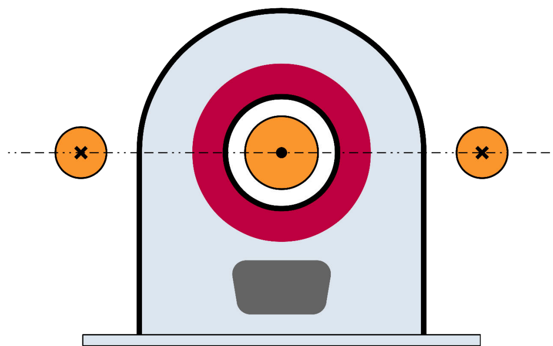
Figure 1-1 Two symmetrical return paths
