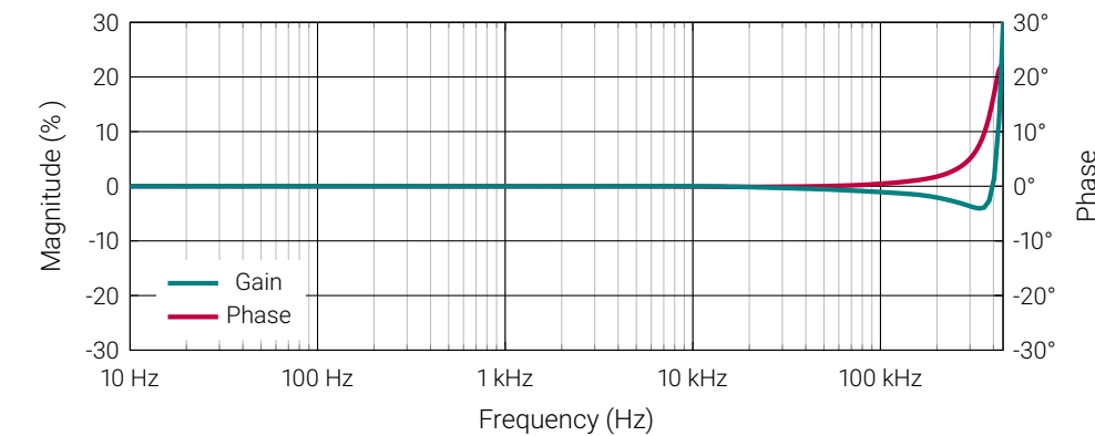
Figure 4: Frequency characteristics
