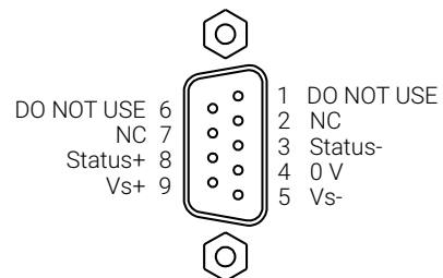
Figure 4: D-sub-9 connection pinout
