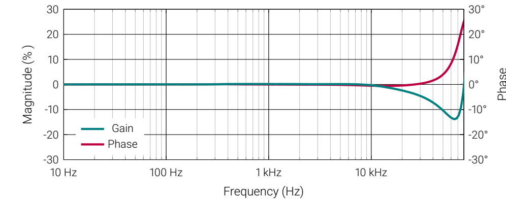
Figure 4: Frequency characteristics
