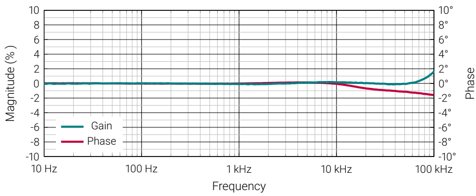
Figure 3: Frequency characteristics
