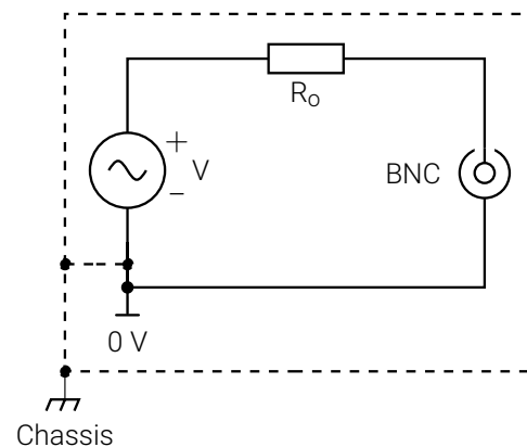
Figure 6: BNC shield and chassis connection
