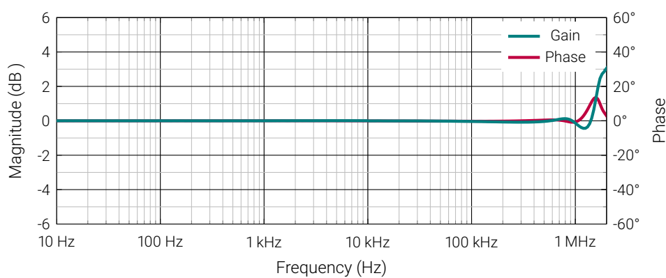
Figure 4: Frequency characteristics. For high frequency measurement, see https://danisense.com/wp-content/uploads/Current-Measurements-at-High-Frequencies.pdf
