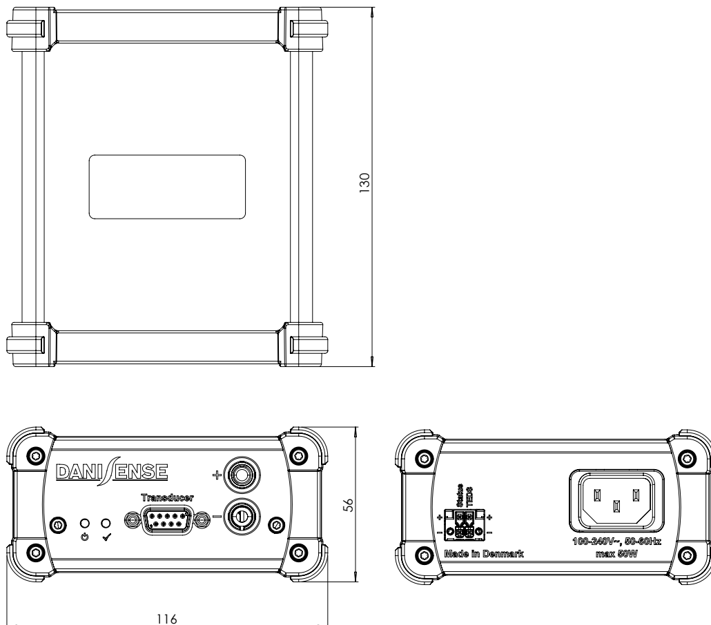
Figure 3: Box dimensions
