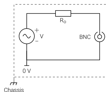
Figure 6: BNC shield and chassis connection
