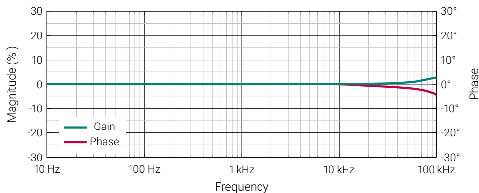
Figure 3: Frequency characteristics
