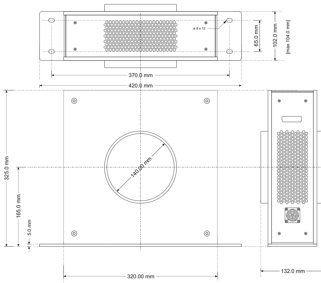
Figure 6: Dimensions of transducer head. 0.3 mm Tolerance
