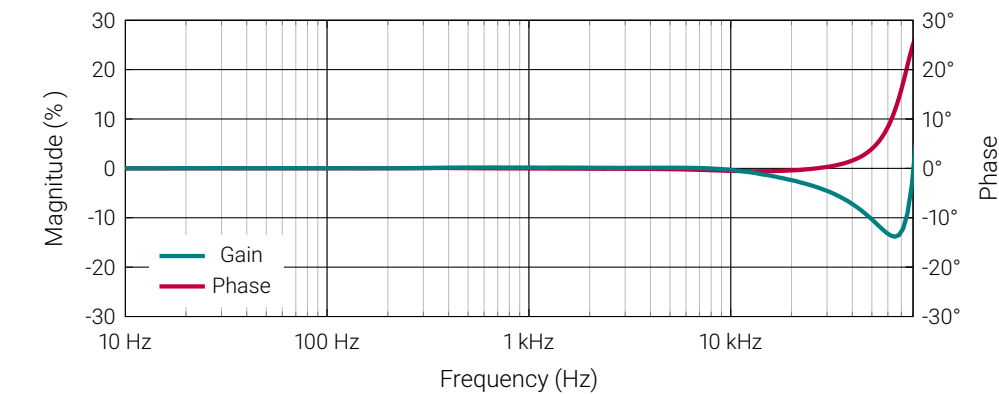
Figure 4: Frequency characteristics
