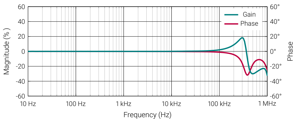
Figure 5: Frequency characteristics
