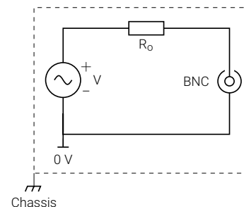
Figure 6: BNC shield and chassis connection
