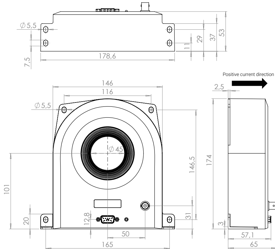
Figure 5: Dimensions of sensor head in mm. General tolerance is 0.3 mm.
