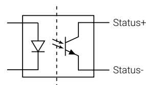
Figure 8: Status signal optocoupler
