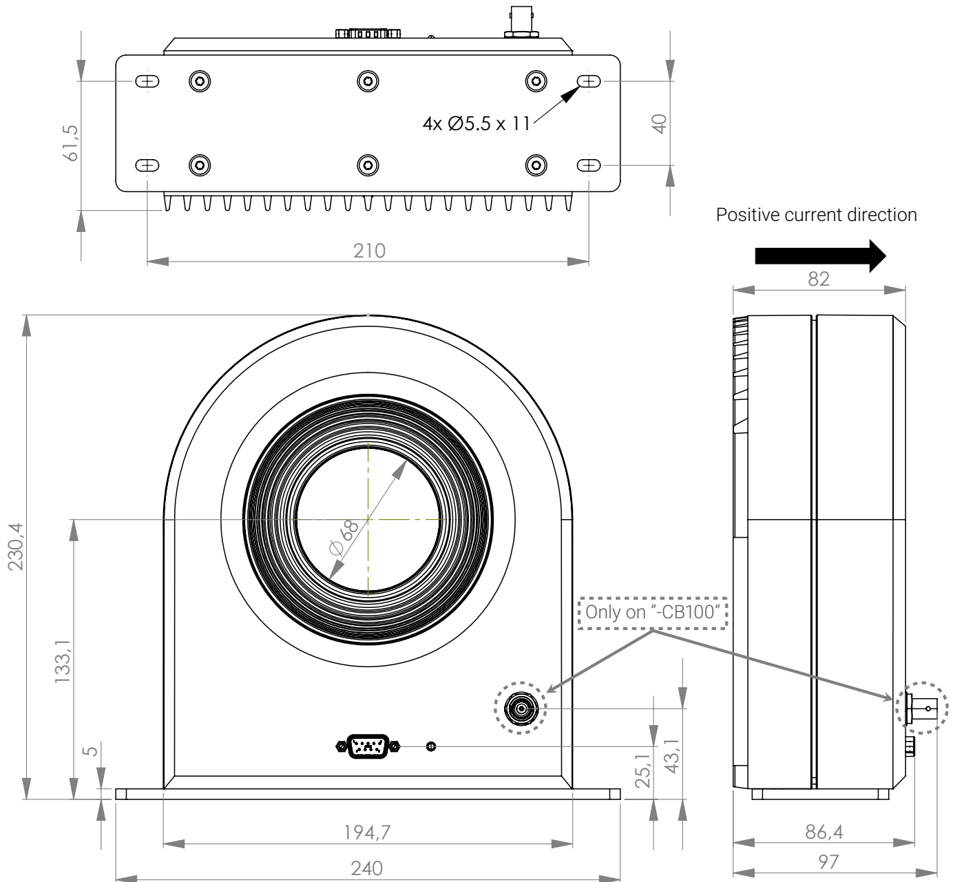
Figure 5: Dimensions of transducer in mm. General tolerance: 0.3 mm.
